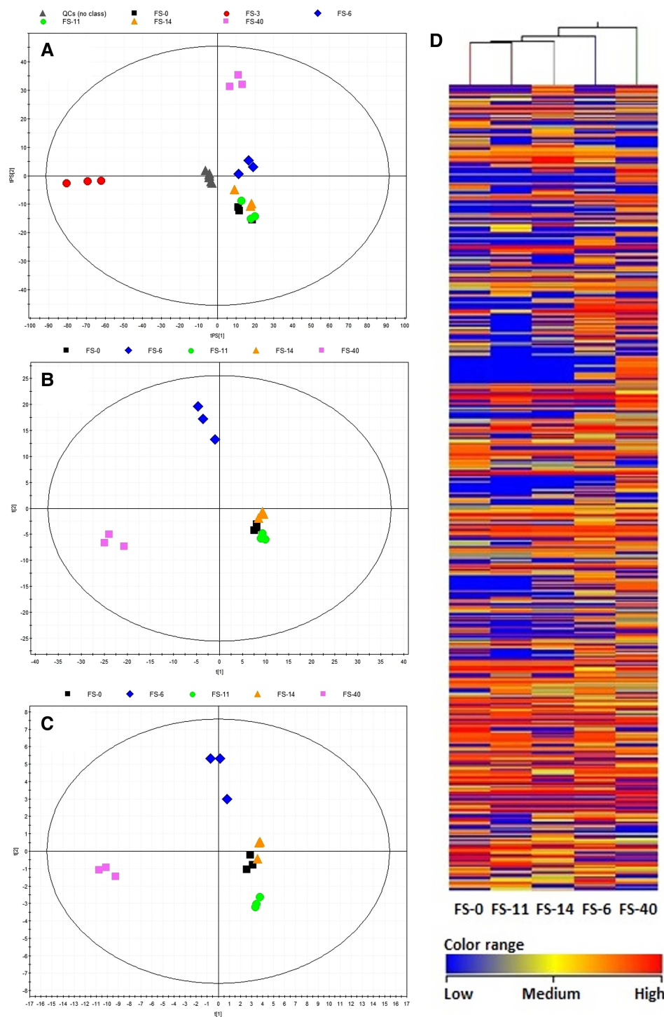
Figure 4 Partial least-squares discriminant analysis score plots and clustering analysis of metabolite profiles after different comparisons. (A) The whole dataset (8600 features) with the prediction for quality control (QC) samples, seven components, R^2=0.989 , Q^2=0.670 ; the robustness of the analytical procedure was demonstrated by the tight clustering of the QC samples. (B) Discriminant variables identified by comparing samples in a pairwise fashion (382 discriminant features from 988 of the 4349 initial variables that were present in all three replicates of samples from any group), four components, R^2=0.978 , Q^2=0.928 . (C) Statistically significant variables identified in the METLIN database (49 features), four components, R^2=0.968 , Q^2=0.915 . (D) The effect of antibiotics on the human gut microbiota, as determined by a two-way hierarchical clustering analysis of the metabolite profiles. Hierarchical clustering was performed with a matrix of the total masses that passed the filtering and statistical treatments for each sample. Less abundant masses in a given community are shown in blue, whereas more abundant masses are shown in red. Note: sample FS-3 was discarded from the analysis due to the presence of faecal material in the cell extracts.
